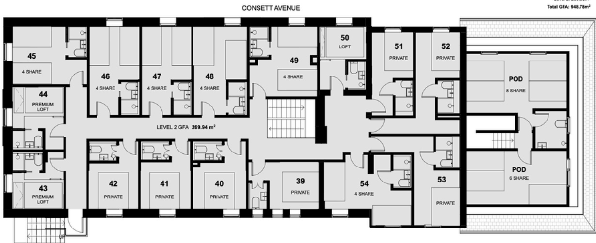
GENERAL ARRANGEMENT PLAN - LEVEL 2 SCALE 1:100@A3
