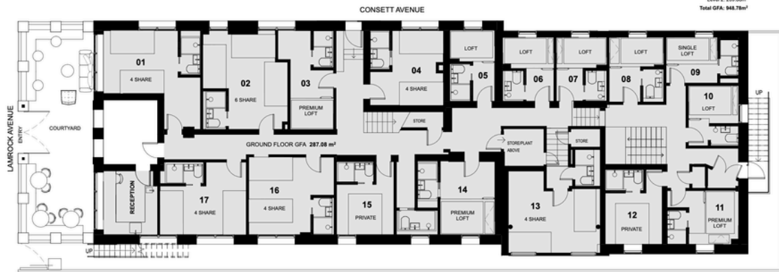
1 GENERAL ARRANGEMENT PLAN - GROUND FLOOR SCALE 1:100@A3
